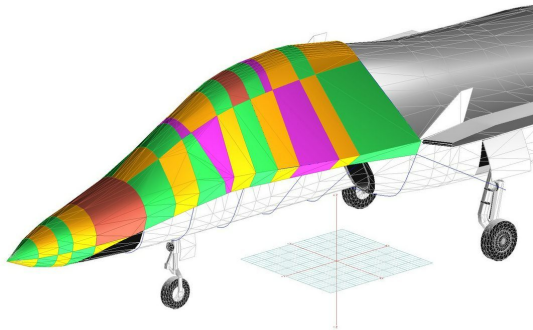
Aermacchi M-346 Canopy/Nose Cover, 3D model
