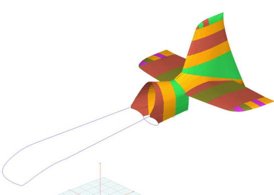
Gamebird GB-1 Extended Canopy/Engine, Wing & Empennage Covers (test fit covers) Gamebird GB-1 Empennage Cover, 3D model
