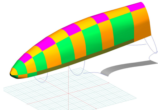
Bede BD-5 Canopy/Nose Cover (3D model)
